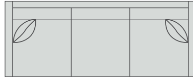
Long Sofa 9 S 2 - 3 W90.5 D38 H33 Inside Seat W84 D22 Std. w/2 P-100 18" Pillows
