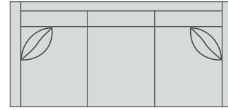
Short Sofa 9 B 1 - 3 W75.5 D38 H33 Inside Seat W69.5 D22 Std. w/2 P-100 18" Pillows
