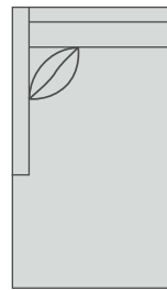
Left Arm Chaise 9 C L - X W33 D64 H33 Inside Seat W30 D49 Std. w/1 P-100 18" Pillow
