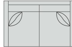
Loveseat 9 L 1 - 3 W60 D38 H33 Inside Seat W53 D22 Std. w/2 P-100 18" Pillows
