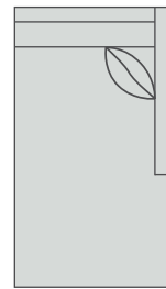
Right Arm Chaise 9 C R - X W33 D64 H33 Inside Seat W30 D49 Std. w/1 P-100 18" Pillow
